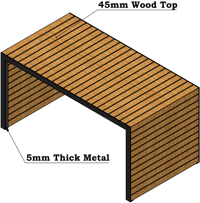
ISO VIEW
